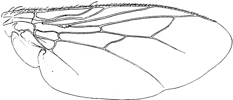
FIGURE 2.— Oligoœstrus œstroideus , new genus and species: Wing
